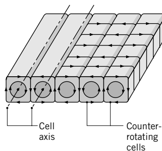
FIGURE 9.11 Longitudinal roll cells characteristic of advection in a horizontal fluid layer heated from below ( 1708 < Ra_L \leq 5 \times 10^4 ).
