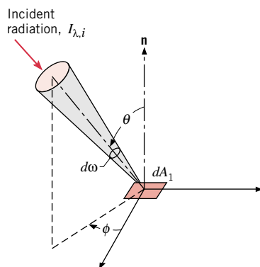
FIGURE 12.9 Directional nature of incident radiation.
