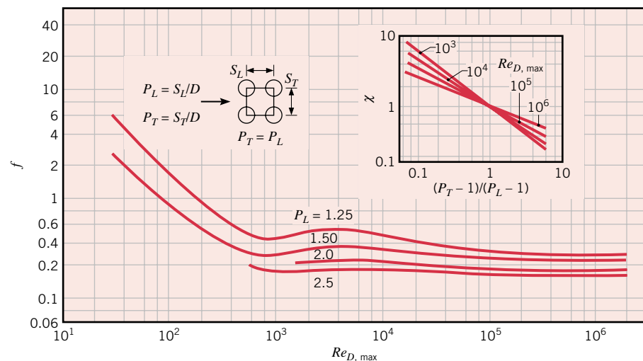
FIGURE 7.13 Friction factor f and correction factor \chi for Equation 7.69. In-line tube bundle arrangement [15]. Used with permission.
