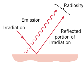
FIGURE 12.10 Surface radiosity.
